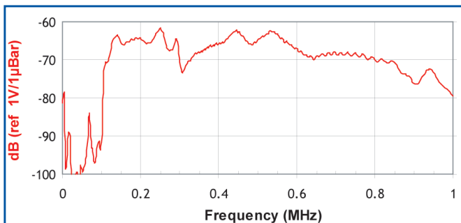
Frequency response of the ISD9203B. Calibration based on ASTM E976.
