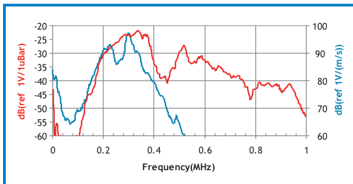
Frequency response of the R30I-AST. Calibration based on ASTM E1106; Calibration based on ASTM E976.
