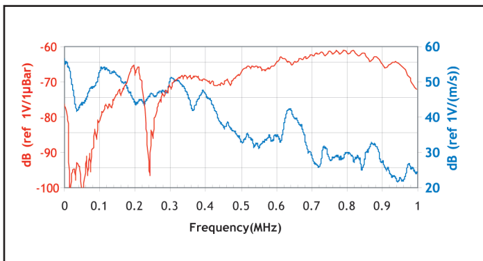
Frequency response of the WS \alpha . Calibration based on ASTM E1106; Calibration based on ASTM E976.
